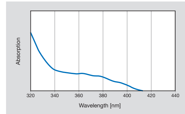
Absorption spectrum of the photoinitiator (wavelength range from 320 to 420 nm) of the UV- and light-curing DELO PHOTOBOND products in an acrylate matrix.
